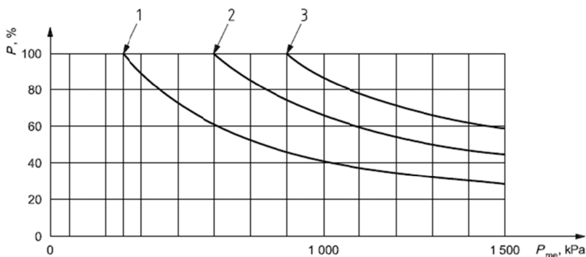
Figure 6 - Guide values for maximum possible sudden power increases as a function of brake mean effective pressure, p_{me} , at declared power (four-stroke engines)
