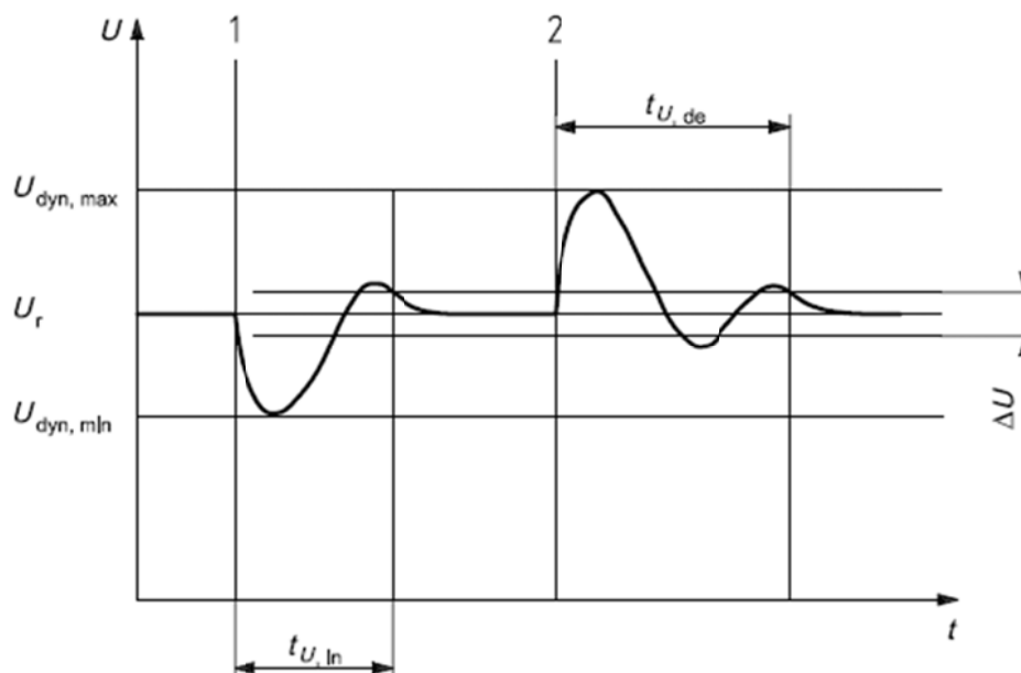
Figure 4 - Dynamic frequency behaviour
